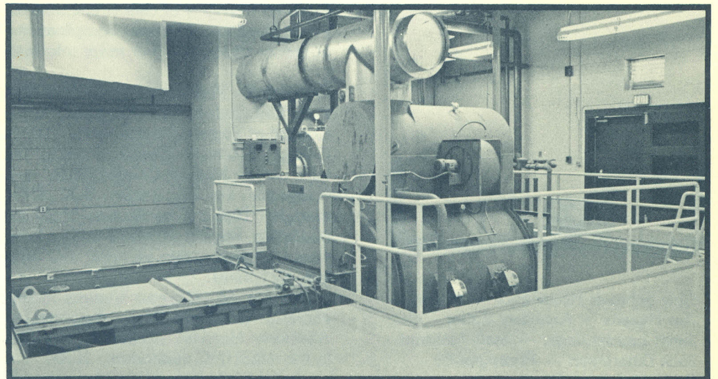
Early in its construction this summer, workers direct the unloading of one of the two incinerator chambers into its new home (left). The finished product, below, enclosed in the GSB. The loading hopper, where trash is placed for burning, is visible at lower left, along the floor.
